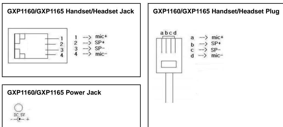
Figure 2: GXP1160/GXP1165 Pin-out
