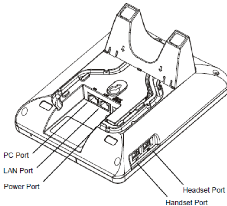
Figure 1: GXP1160/GXP1165 Ports
